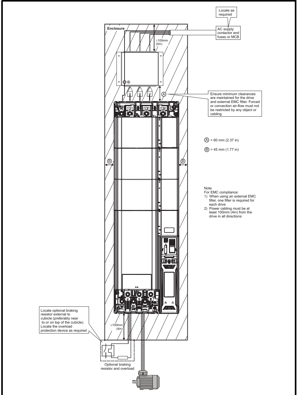
Figure 3-9 Enclosure layout
