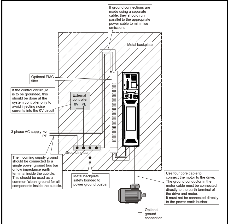
Figure 4-13 General EMC enclosure layout showing ground connections
