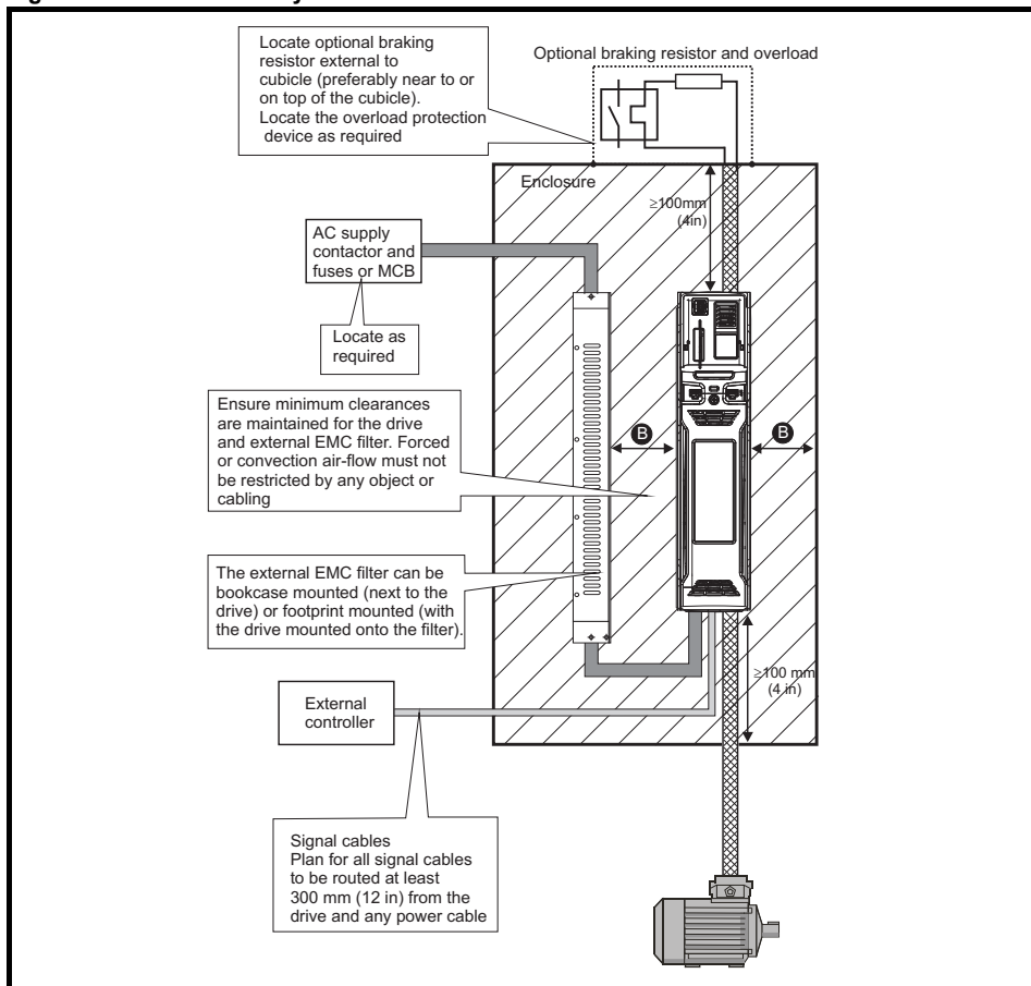
Figure 3-13 Enclosure layout
