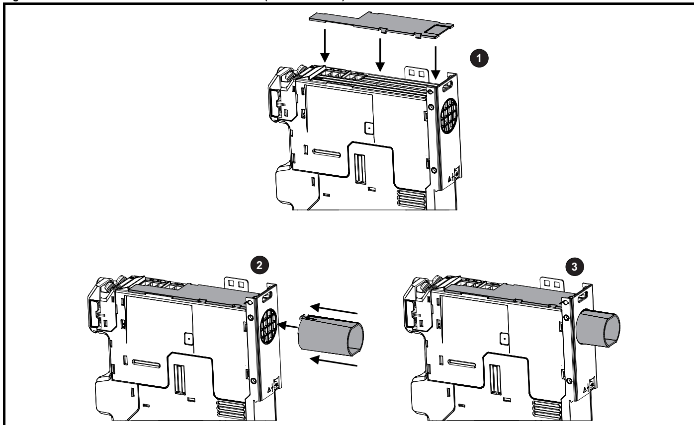
Figure 3-18 Installation of Ultraflow™ rear vent kit (frame 1 shown)
