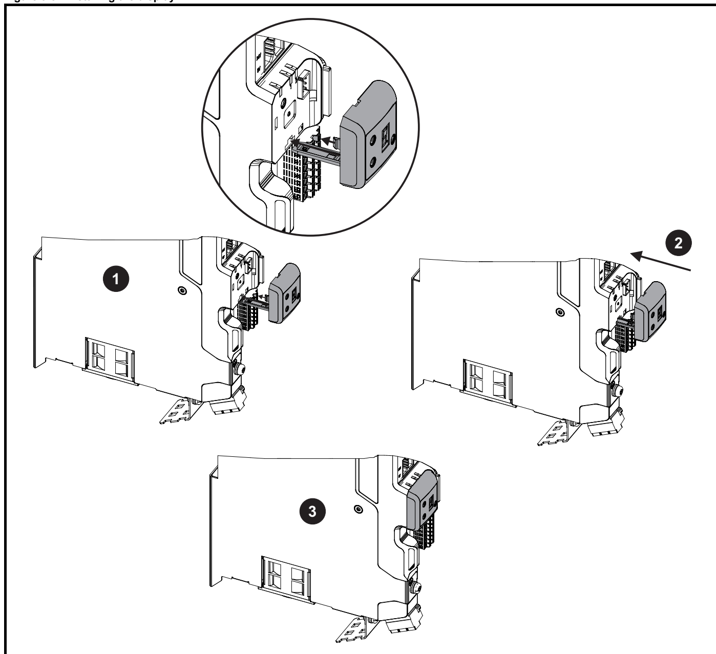
Figure 3-5 Installing the display
