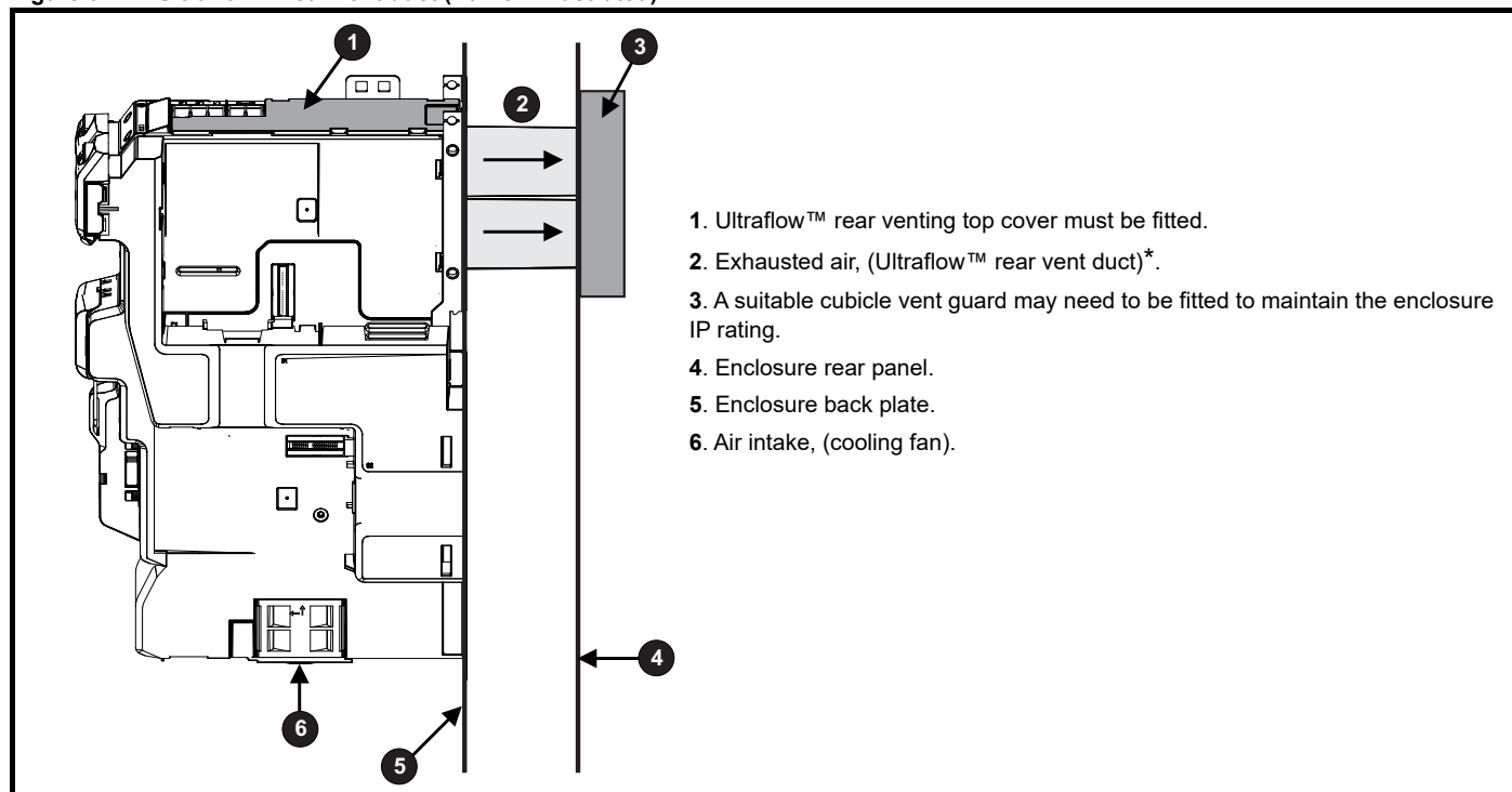
Figure 3-17 Ultraflow™ rear vent duct (frame 2 illustrated)
