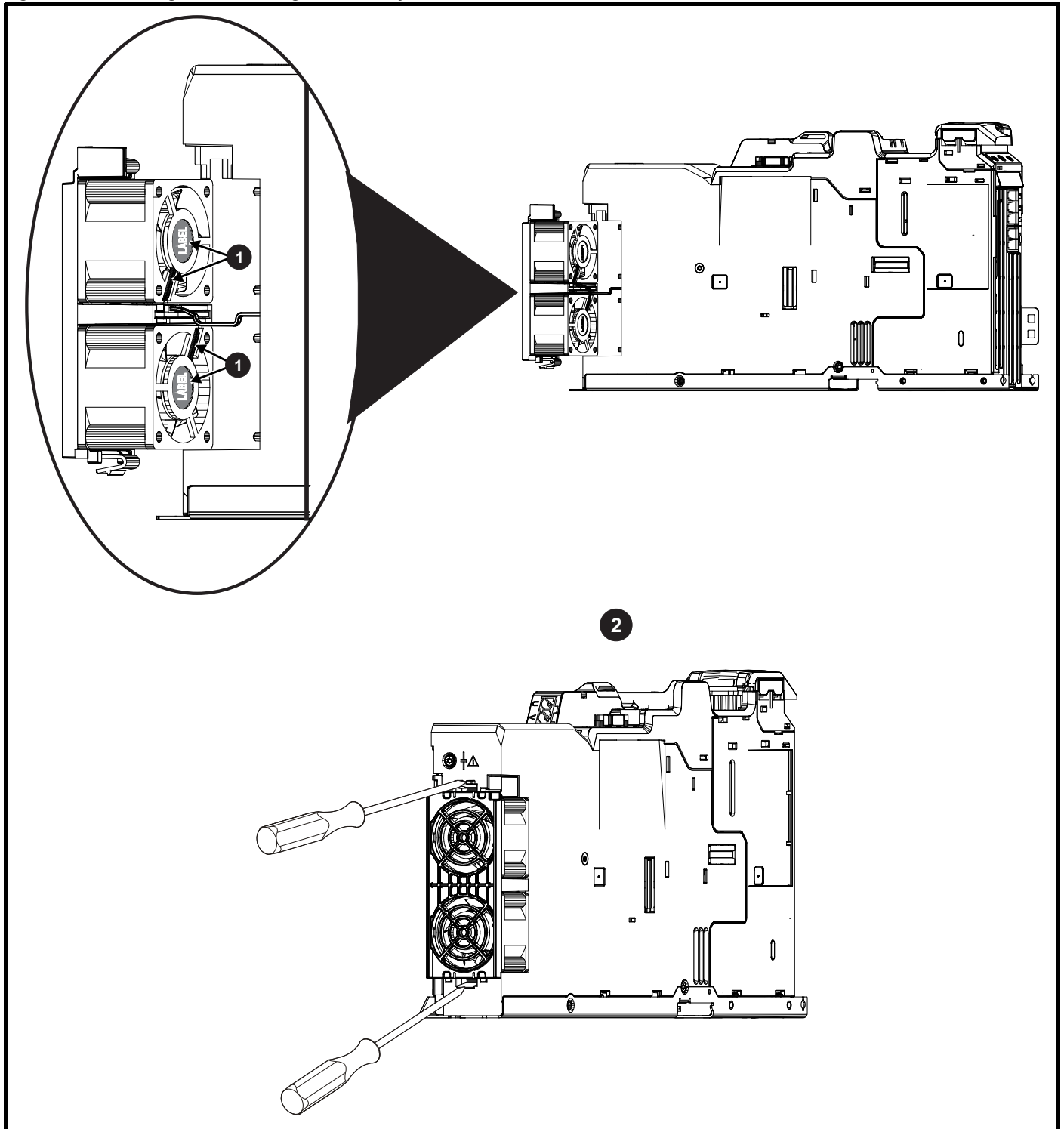
Figure 3-33 Re-fitting frame 3 cooling fan assembly
