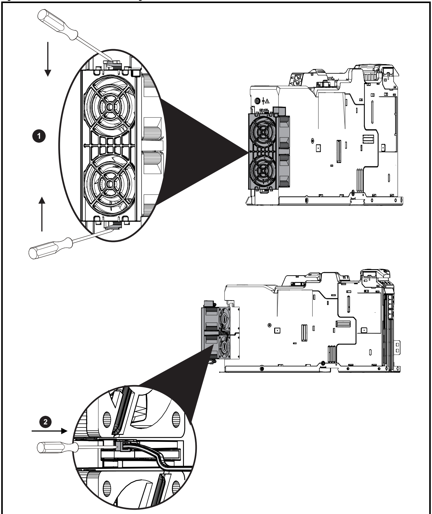
Figure 3-32 Removal of frame size 3 cooling fan
