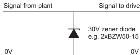
Figure 4-28 Surge suppression for digital and unipolar inputs and outputs
