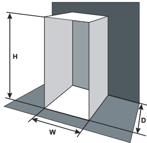
Figure 3-20 Enclosure having front, sides and top panels free to dissipate heat
