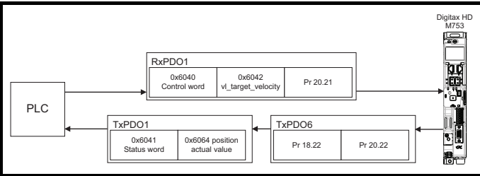
Figure 9-3 EtherCAT PDO configuration
