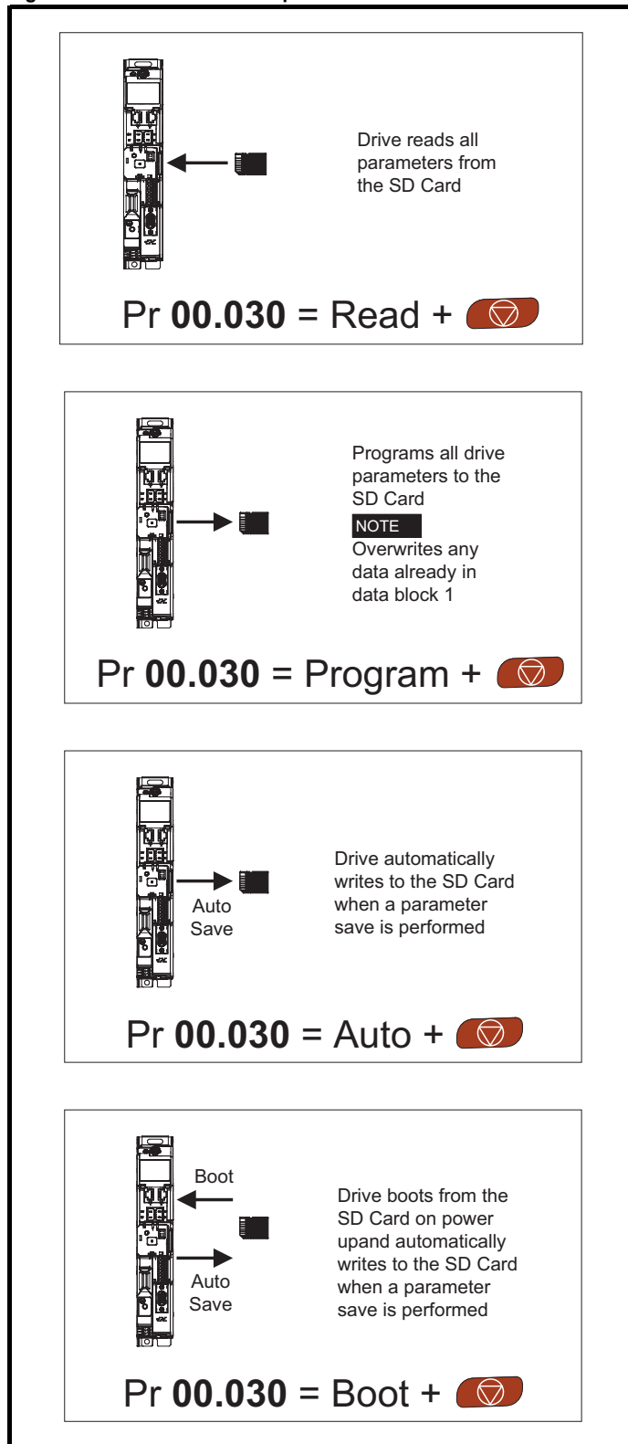
Figure 10-2 Basic SD Card operation
