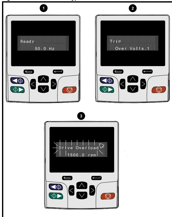
Figure 13-2 KI-Remote Keypad status modes
